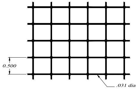
1/2" HARDWARE GALVANIZED HARDWARE CLOTH
