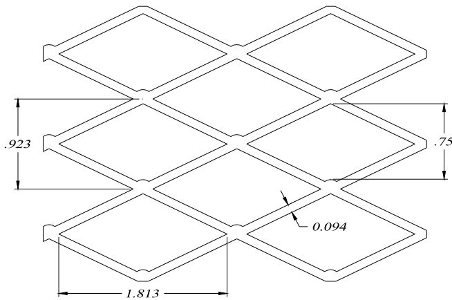
3/4" FLATTENED EXPANDED METAL ALUMINUM BIRD SCREEN .051 THICK
