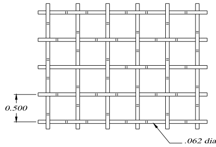
1/2" WOVEN ALUMINUM MESH INTERCRIMPED
