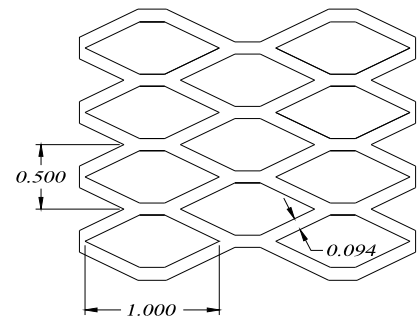
1/2" FLATTENED EXPANDED METAL ALUMINUM BIRD SCREEN .051 THICK
