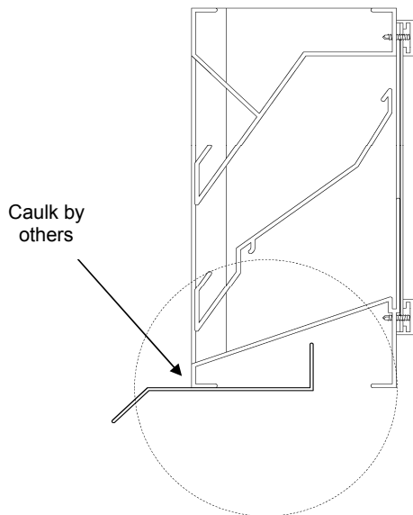
Typical Sill Installation Detail
